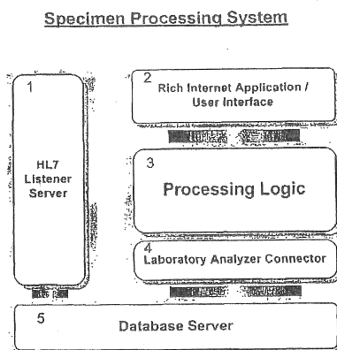
FIG. 4: Specimen Processing System
